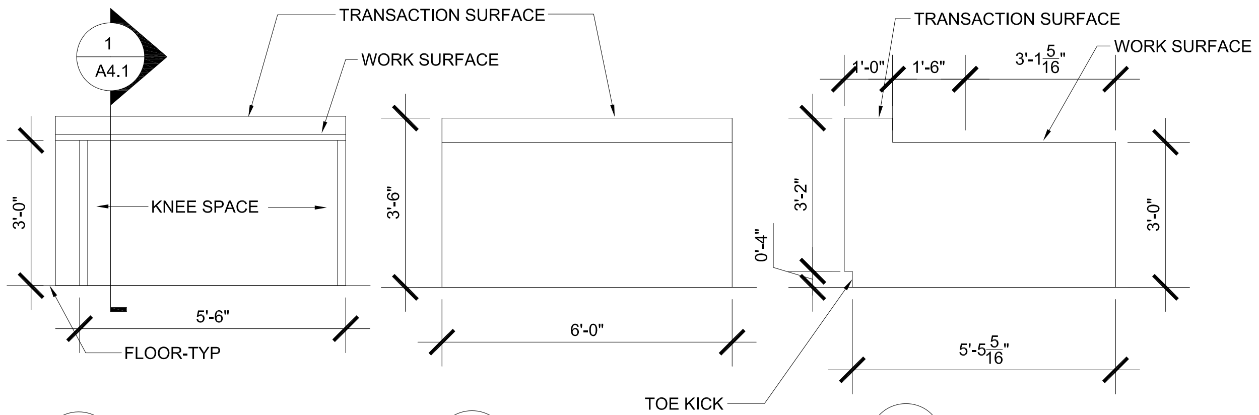
1 BACK ELEVATION \frac{1}{2}'' = 1'-0''
