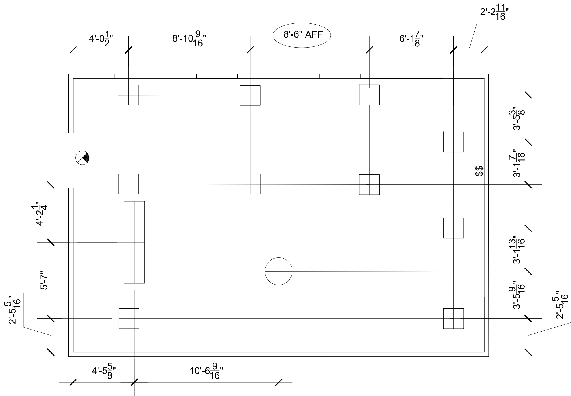
1 REFLECTED CEILING PLAN - SECOND FLOOR
