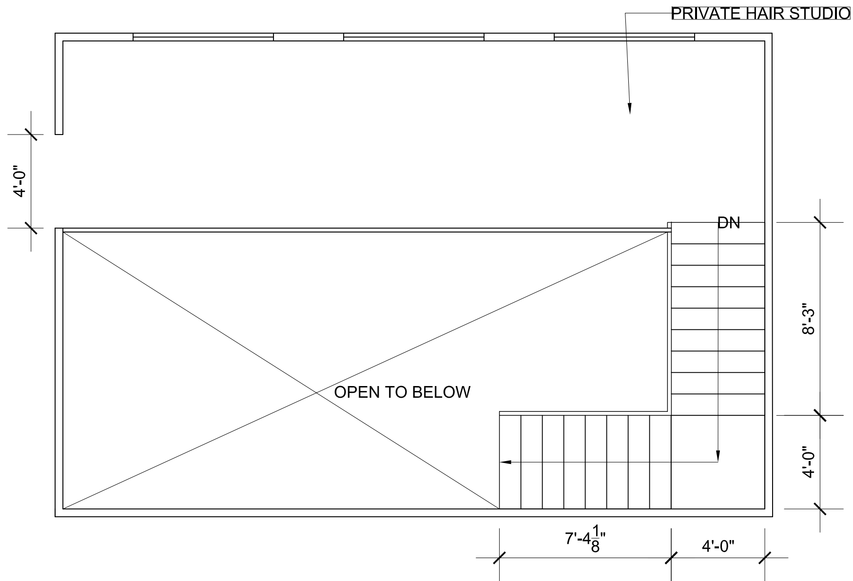
1 PARTITION PLAN - SECOND FLOOR \frac{1}{4}'' = 1'-0''
