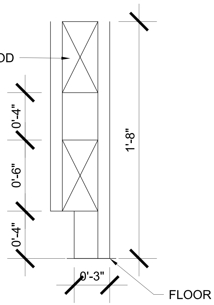
2 DETAIL 3" = 1'-0"
