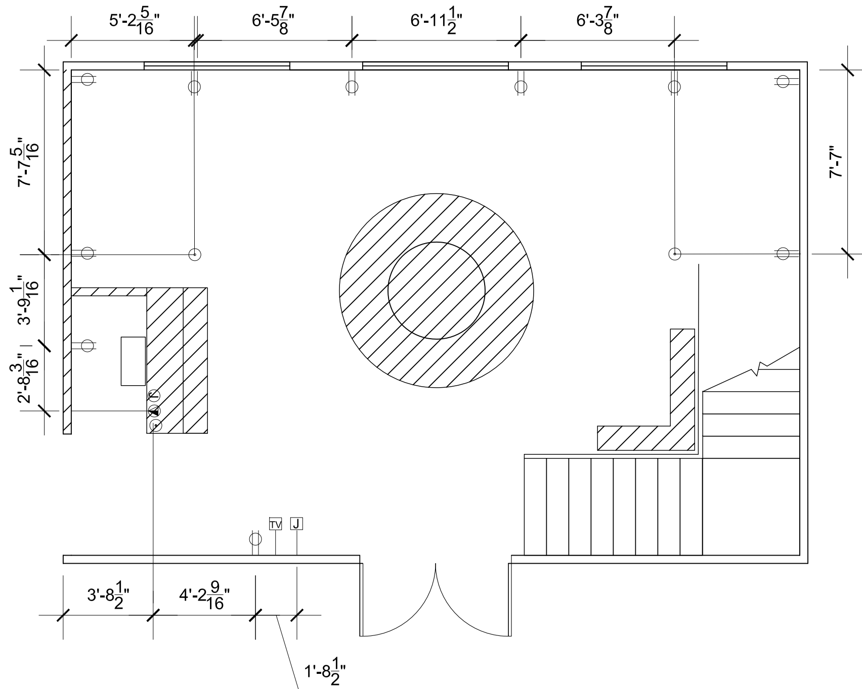
1 POWER AND TELECOM PLAN - FIRST FLOOR \frac{1}{4}'' = 1'-0''
