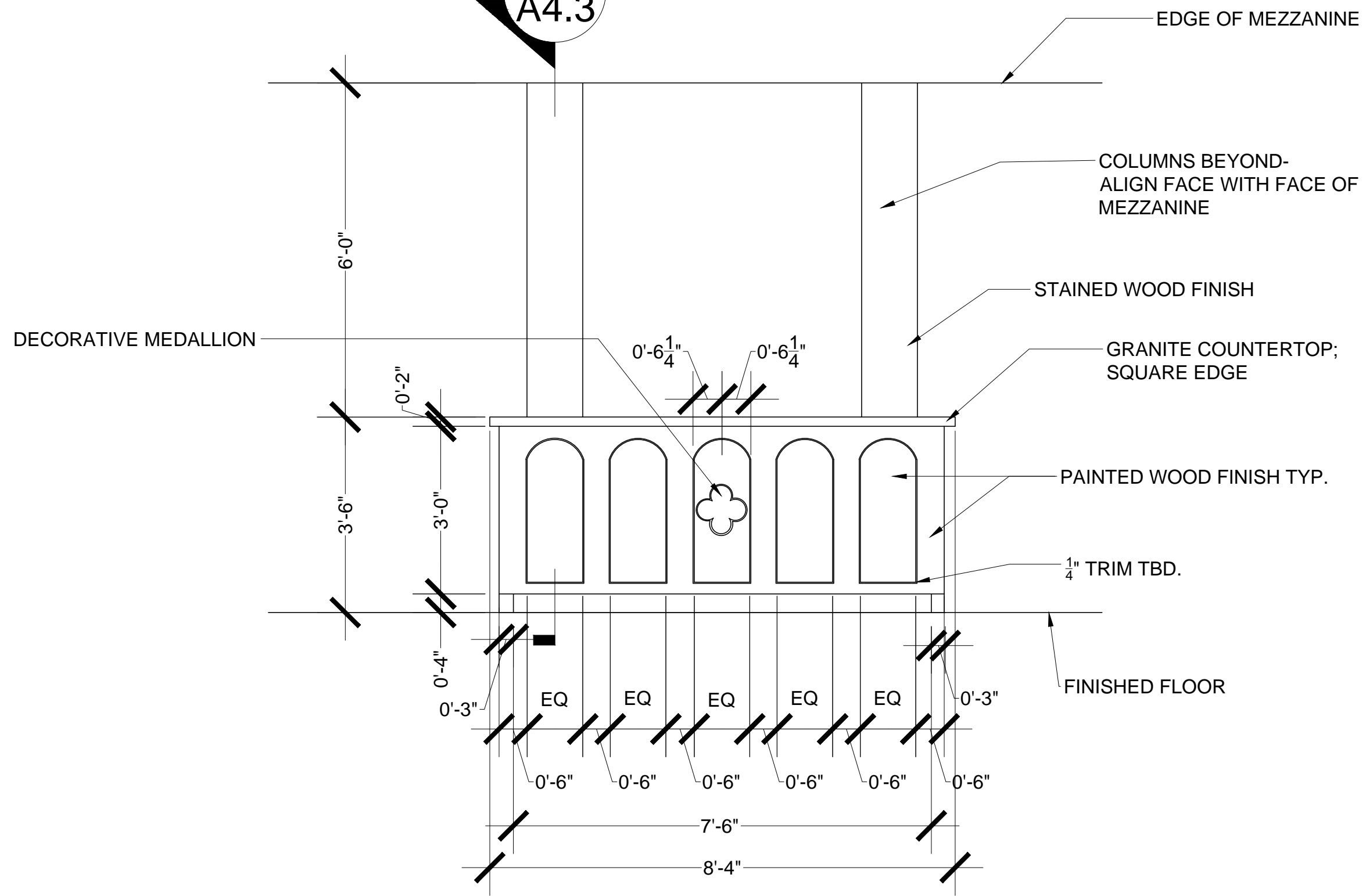
1 ELEVATION PLAN- FRONT VIEW SCALE: 0'-1/2" = 1'-0"
