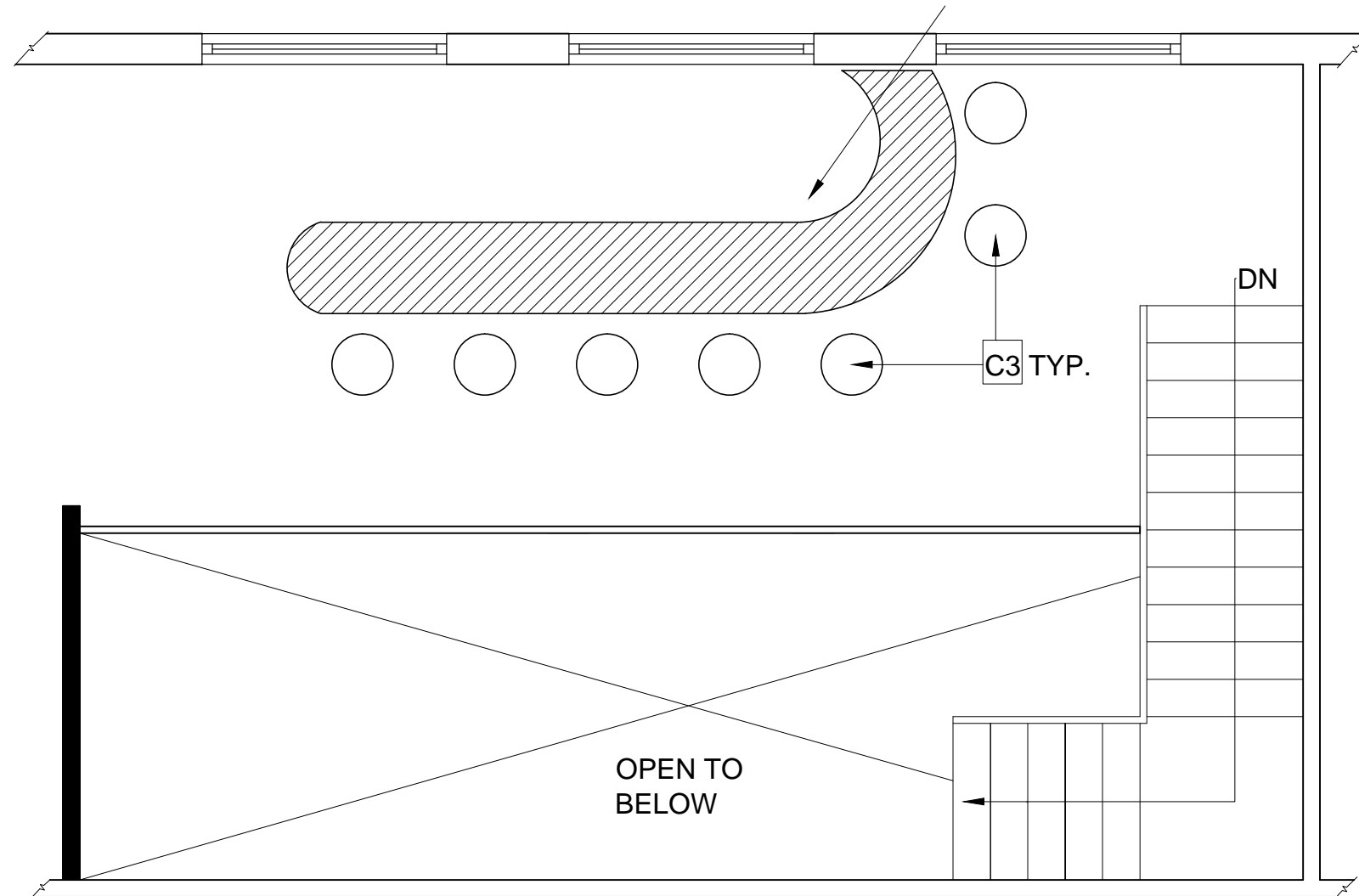
① FURNITURE PLAN 2ND FLOOR SCALE: 0'- \frac{1}{4} " = 1'-0"
