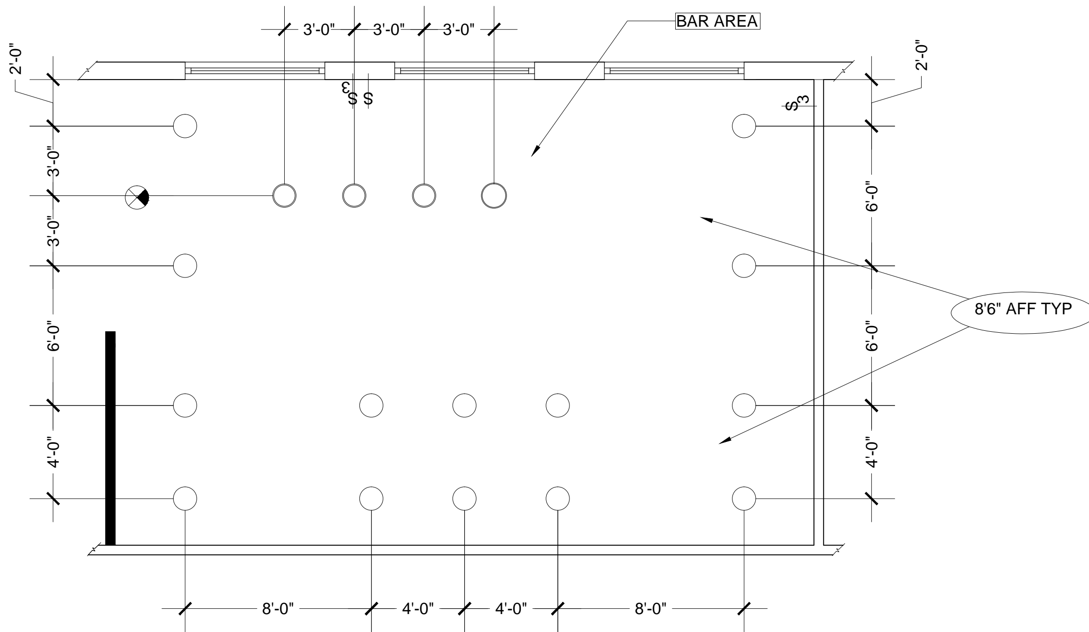
① REFLECTED CEILING PLAN 2ND FLOOR SCALE: 0'- \frac{1}{4} " = 1'-0"
