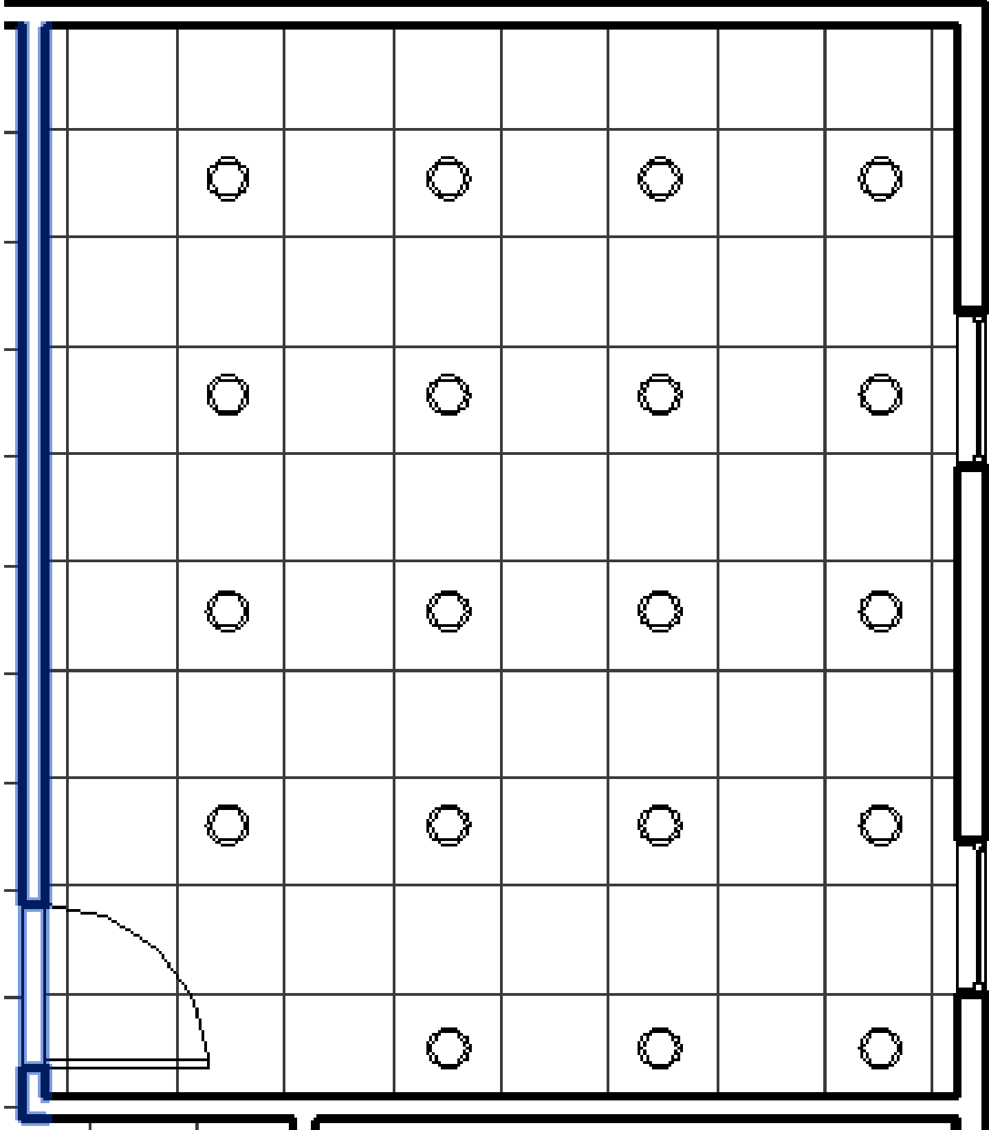
Reflected Ceiling Plan of Conference Room (not to scale)
