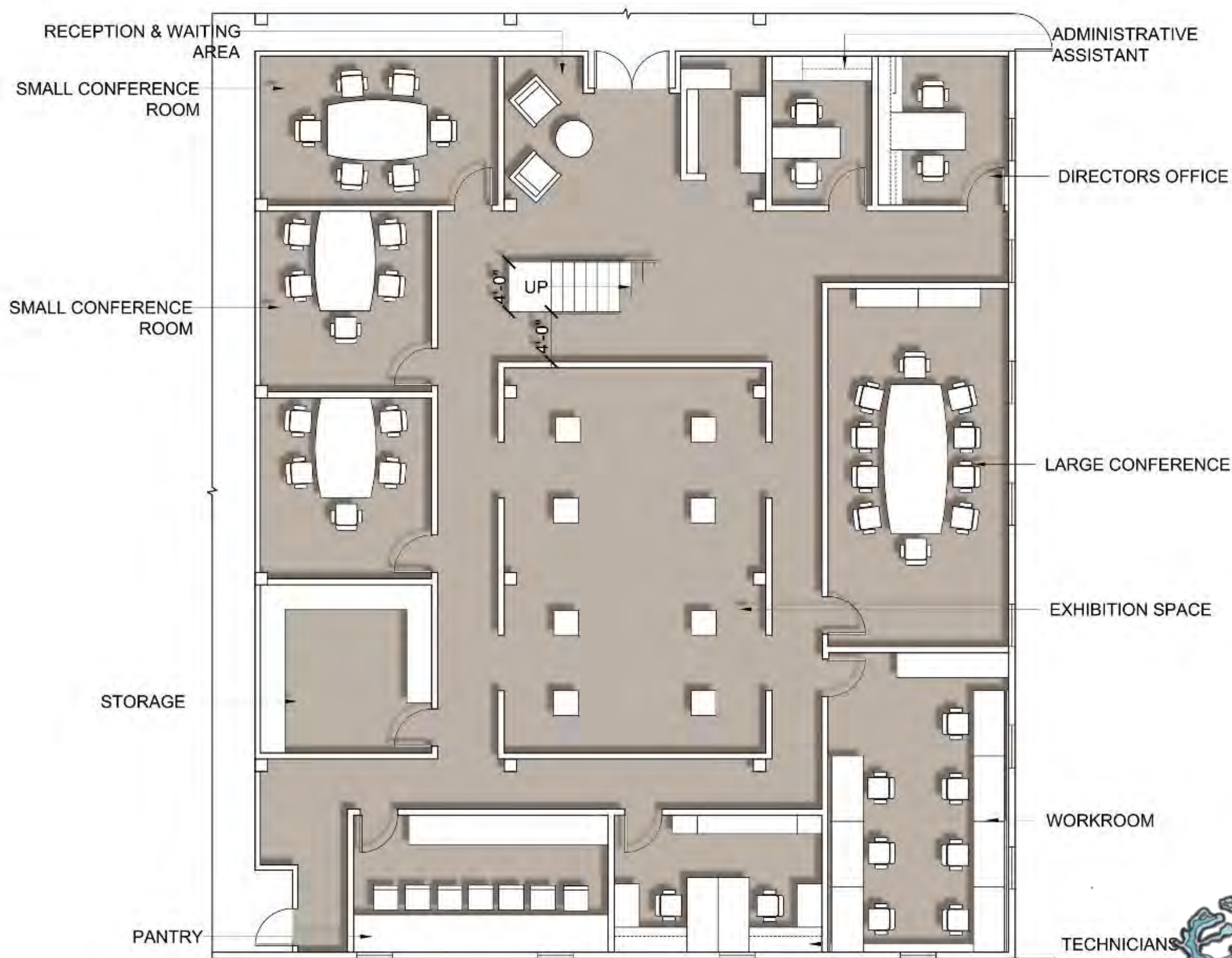
DRAWING IS TO SCALE 1/8" = 1'
