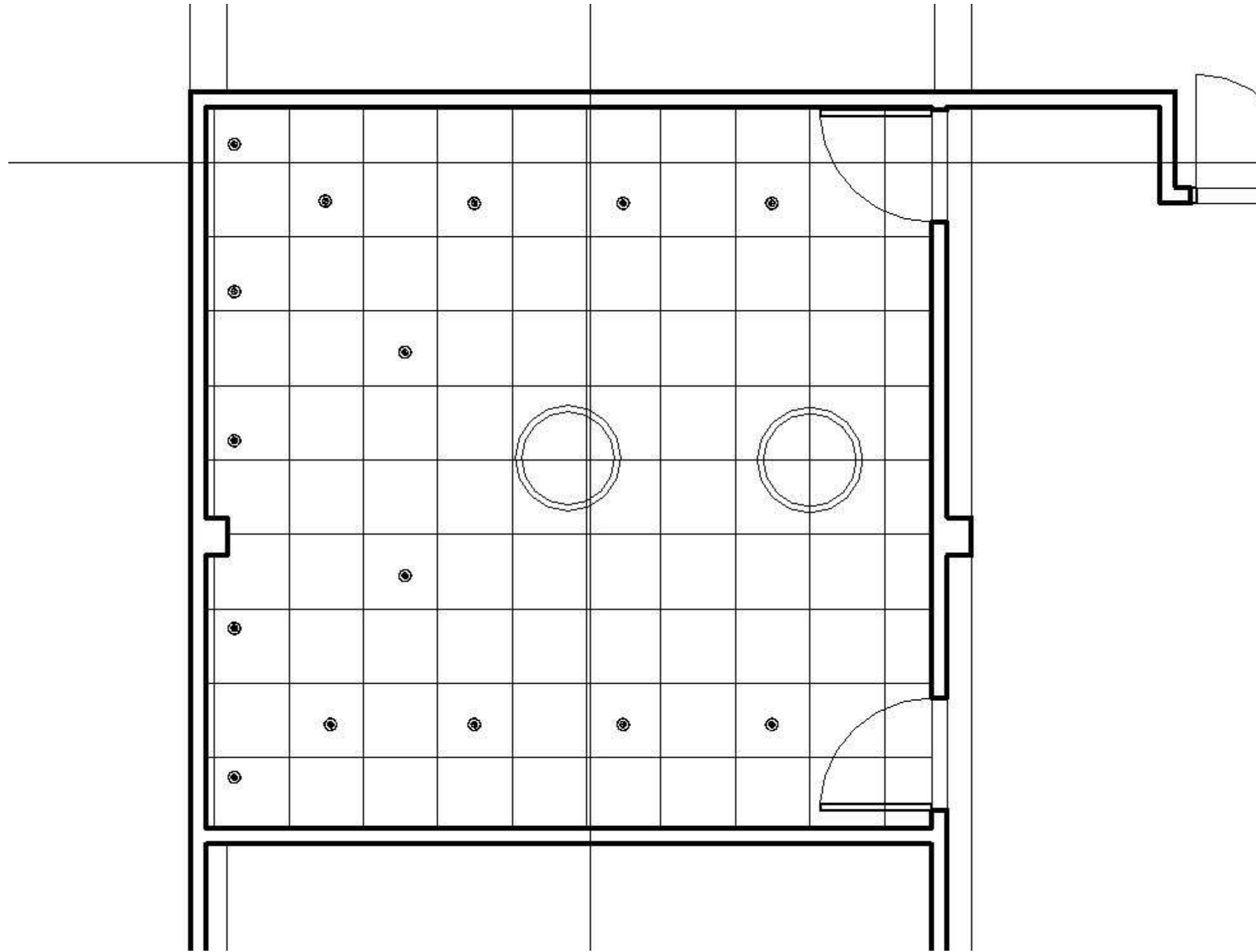
Reflected Ceiling Plan of Conference Room in Revit
