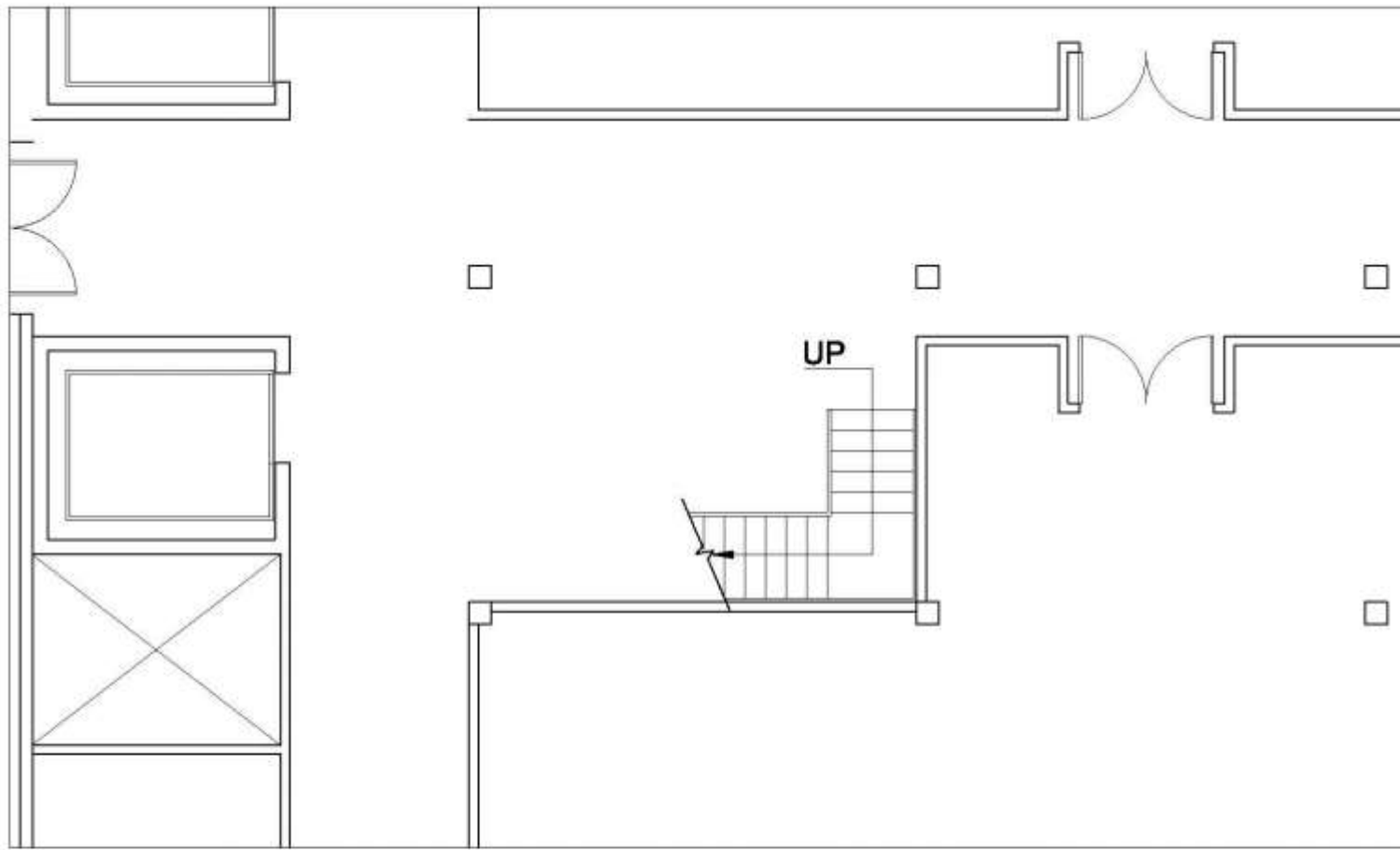
1ST FLOOR
