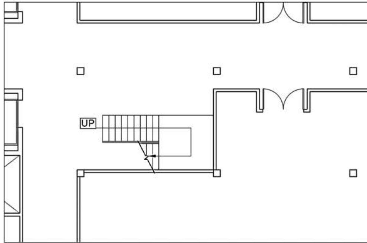
FIRST FLOOR
