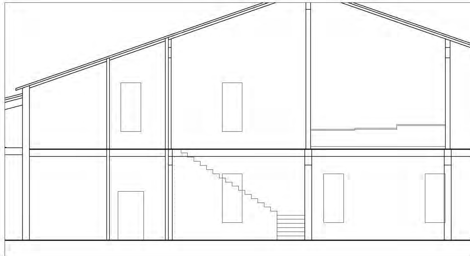
Section
