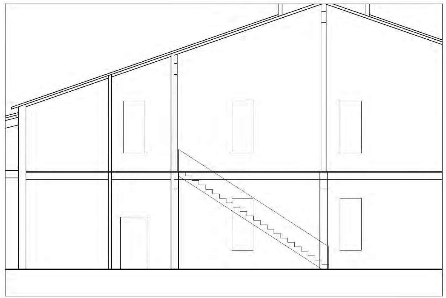
SECTION VIEW
