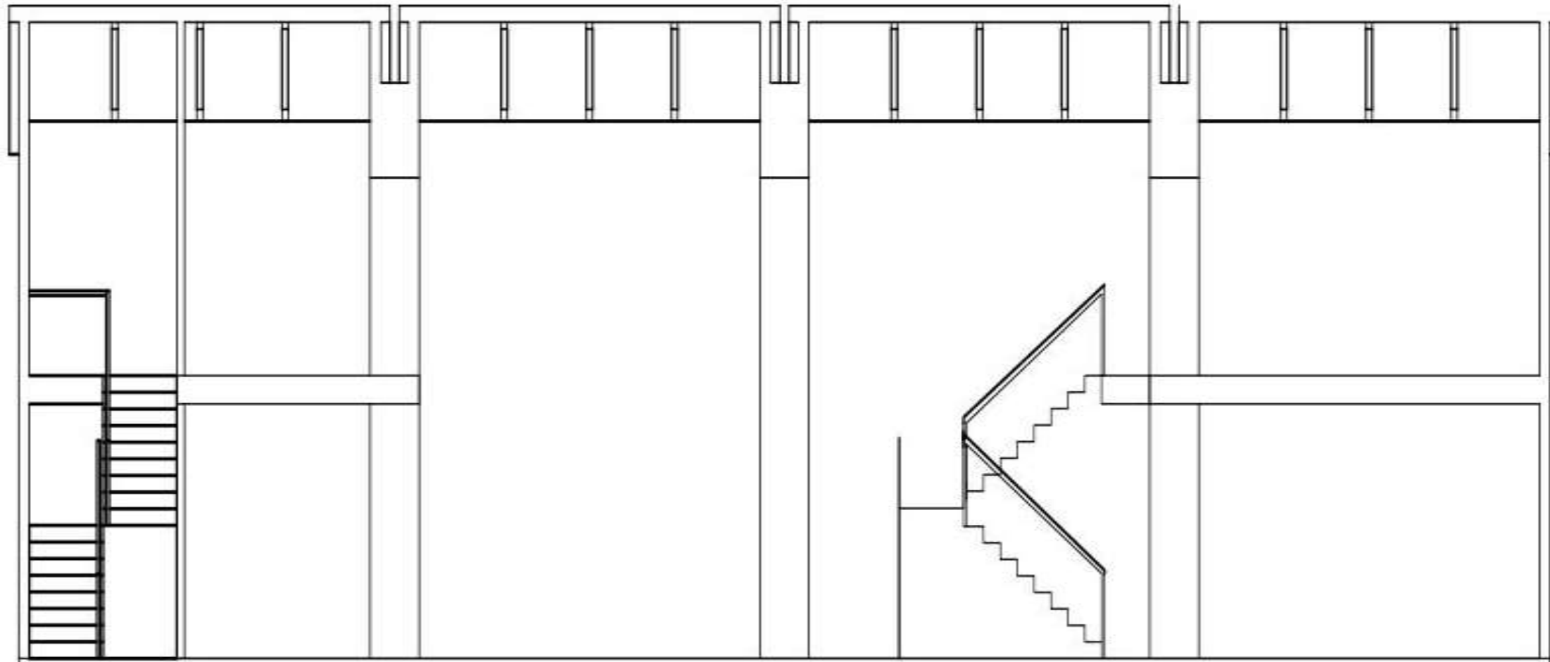
East or West Section
