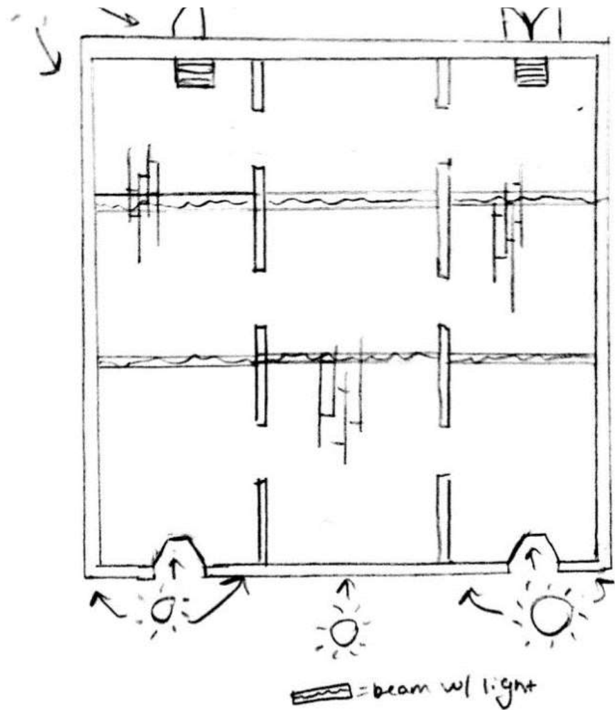
Ceiling/Daylighting #2 Sketched Plan
