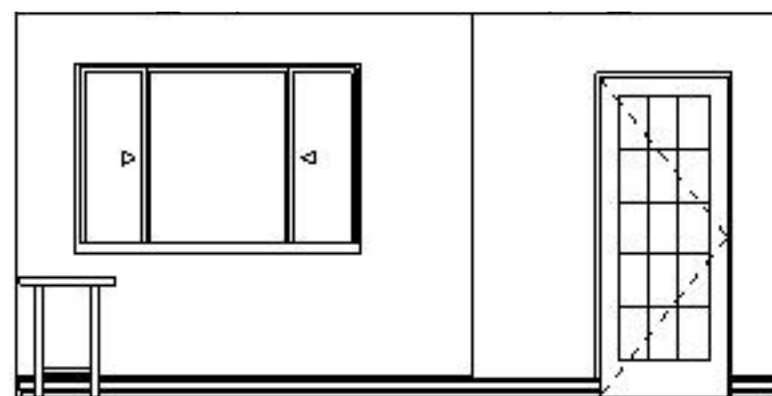
② Primary Bedroom 2 1/4" = 1'-0"
