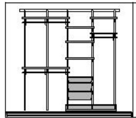
⑧ Second Bedroom Closet 1/4" = 1'-0"
