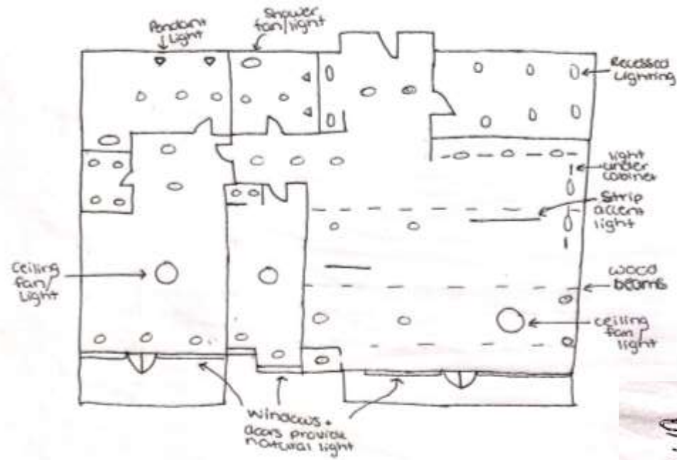
Plan 1
