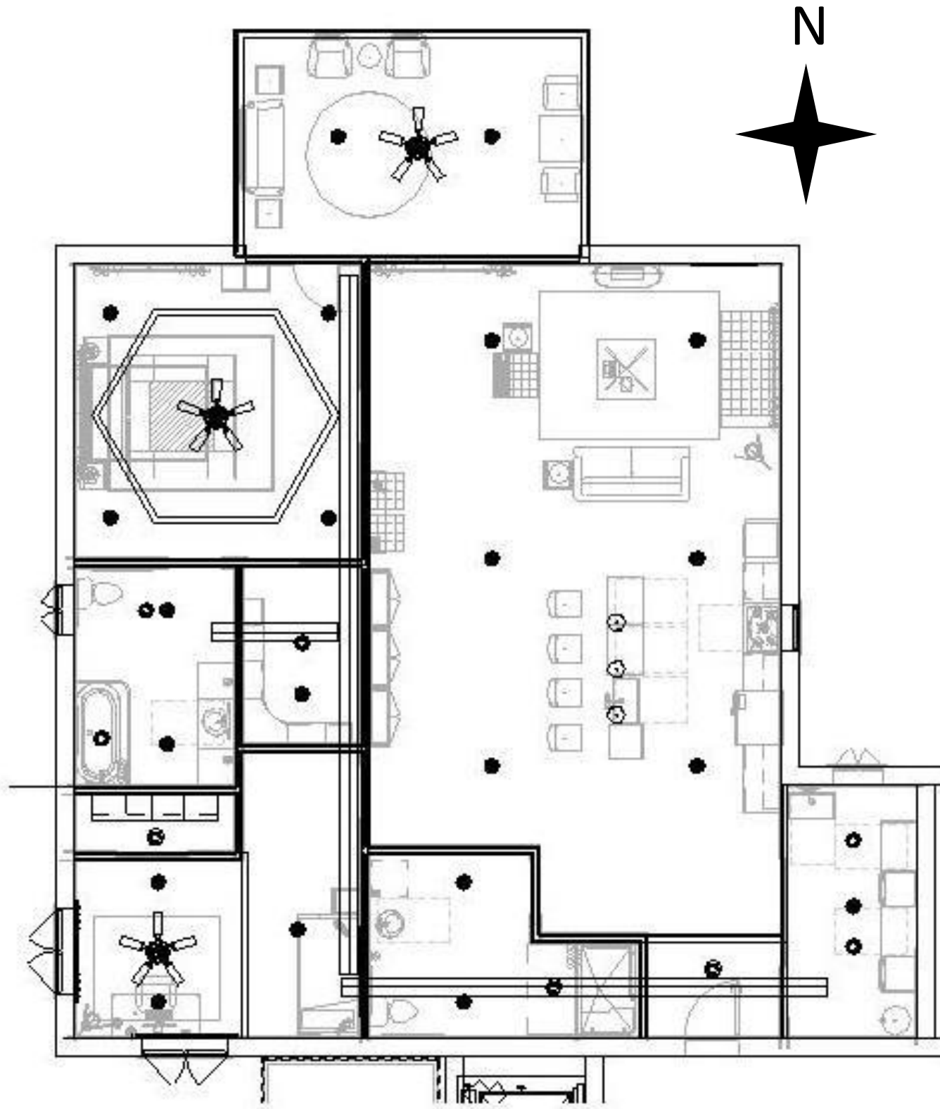
① Reflected Ceiling Plan 1/8" = 1'-0"
